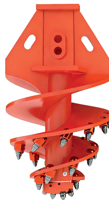
Double start double flight conical auger
